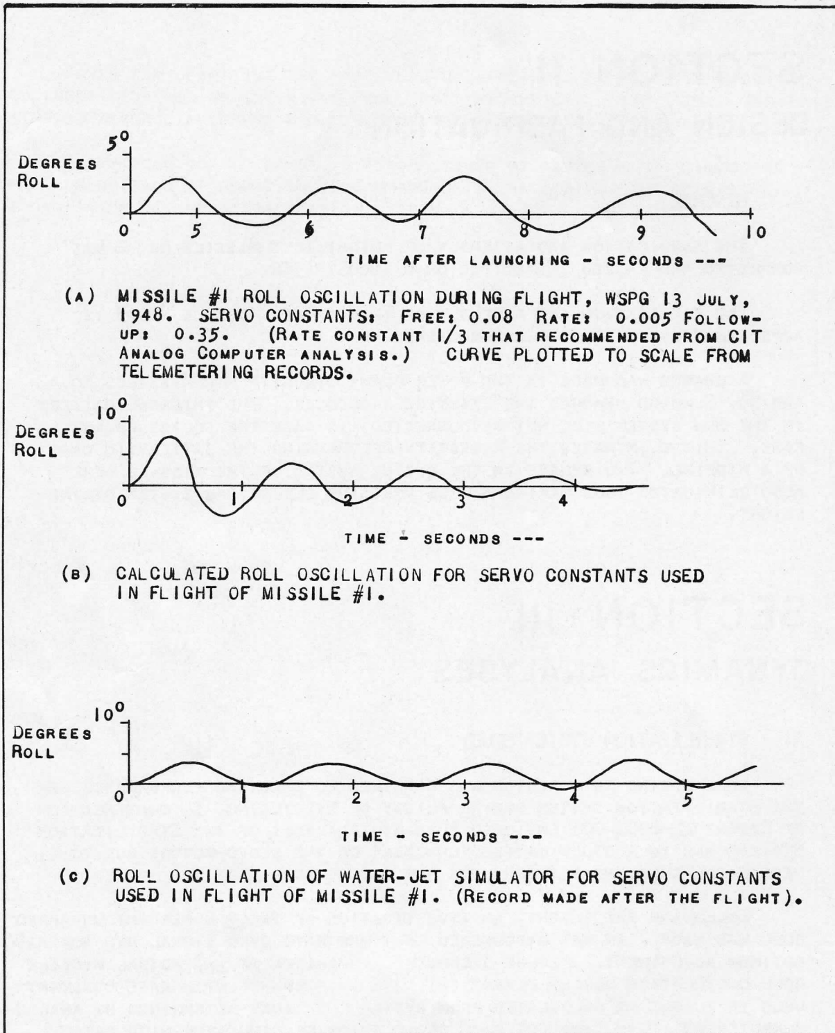
FIG. 5. - MX-774 COMPARISONS OF ROLL OSCILLATIONS
